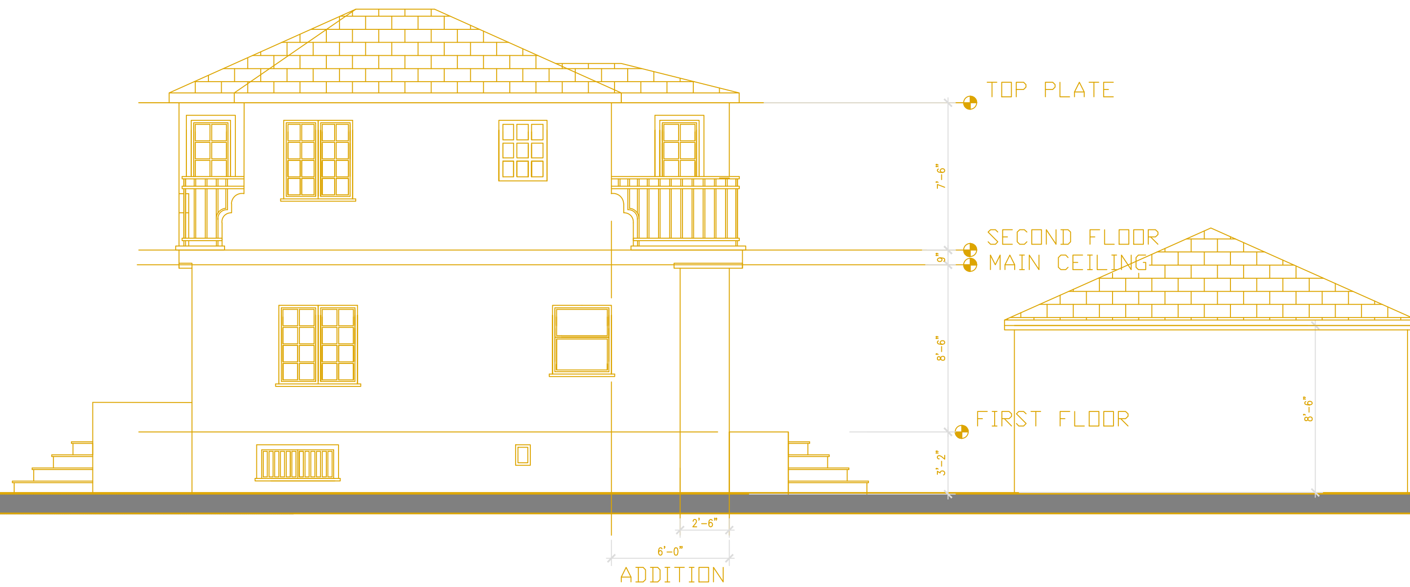
1 NEW RIGHT SIDE ELEVATION A-3.0
